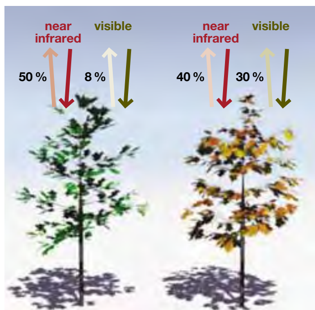
Figure 37: Radiation reflected by plants in satellite images
